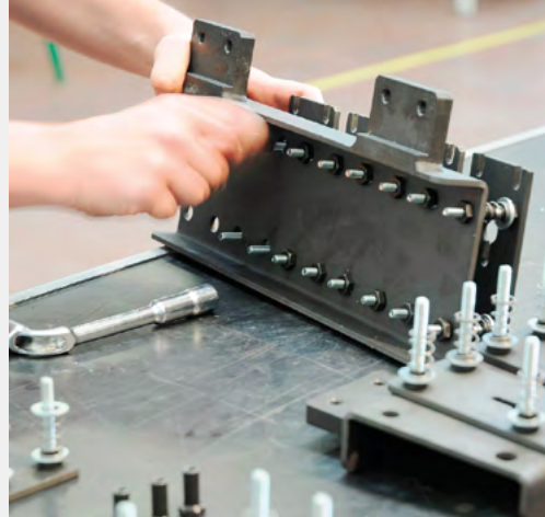
Mechanical assembly
